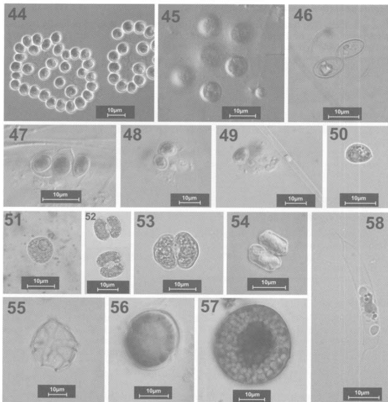
Figs 44-58. 44. Dictyosphaerium pulchellum Wood (in phase contrast). 45. Sphaerocystis (?) sp. 46. Oocystis lacustris Chod. 47-50. Tetraedron sp. [47. with Lugol, 49. with Fragilaria danica (Kütz.) Lange-Bert.] 51. Siderocelis irregularis Hind. 52. Cosmarium cf. laeve Rabenh. 53. Cosmarium sp. 54. Cosmarium cf. regnellii Wille 55. Peridinium umbonatum Stein. 56. Peridinium sp. 57. Gymnodinium sp. (with gentian violet). 58. Urosolenia sp.
