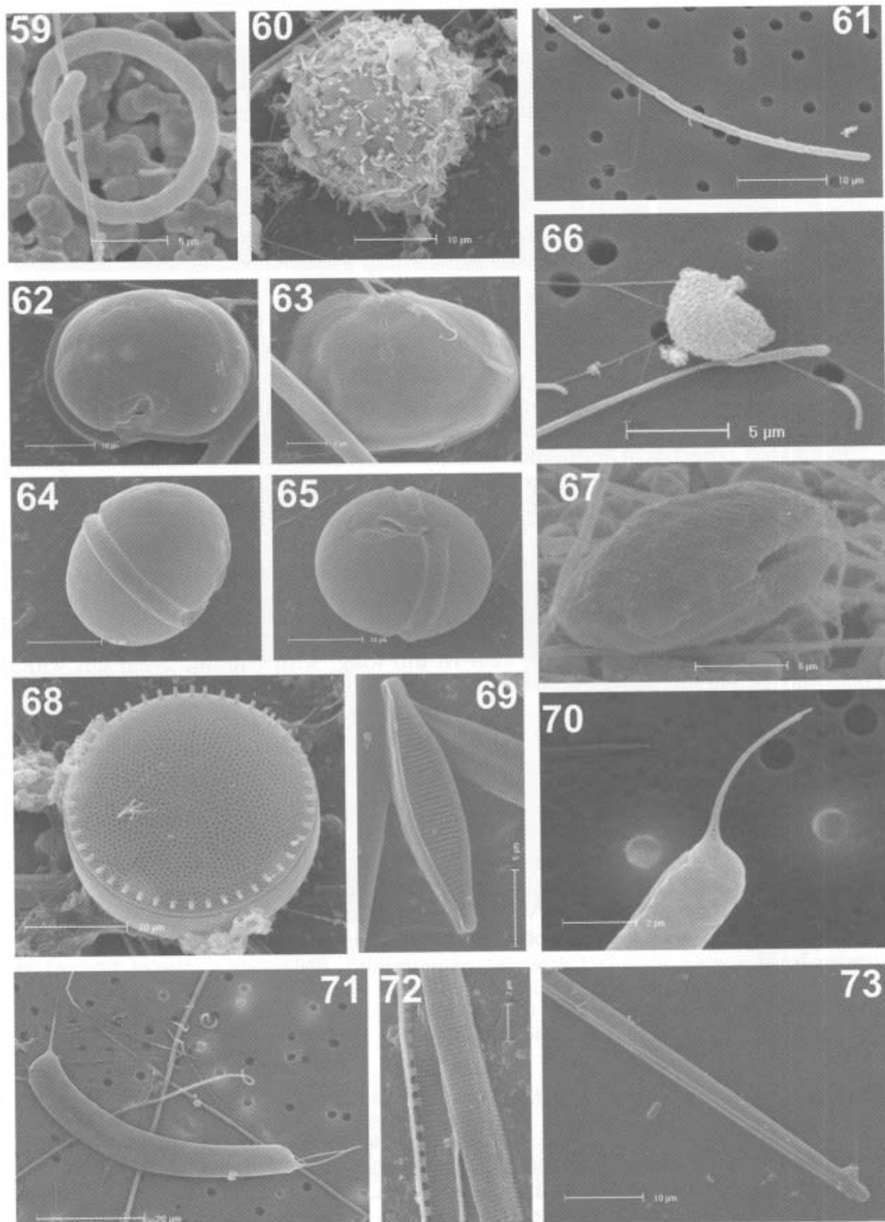
Figs 59-73. 59. Cylindrospermopsis cf. curvispora Wat. 60. Paraphysomonas vestita Stokes 61. Pseudanabaena moniliformis Kom. et Kling. 62-63. Peridinium umbonatum Stein. 64-65. Peridinium sp. 66. Tetraedron sp. 67. Cryptomonas sp. 68. Thalassiosira rudolfi (Bach.) Hasle. 69. Nitzschia fonticola Grun. 70-71. Urosolenia sp. (70. detail of the calyptra with poroids on the process base). 72-73. Nitzschia bacata Hust. (72. detail of fibulae median interruption).
