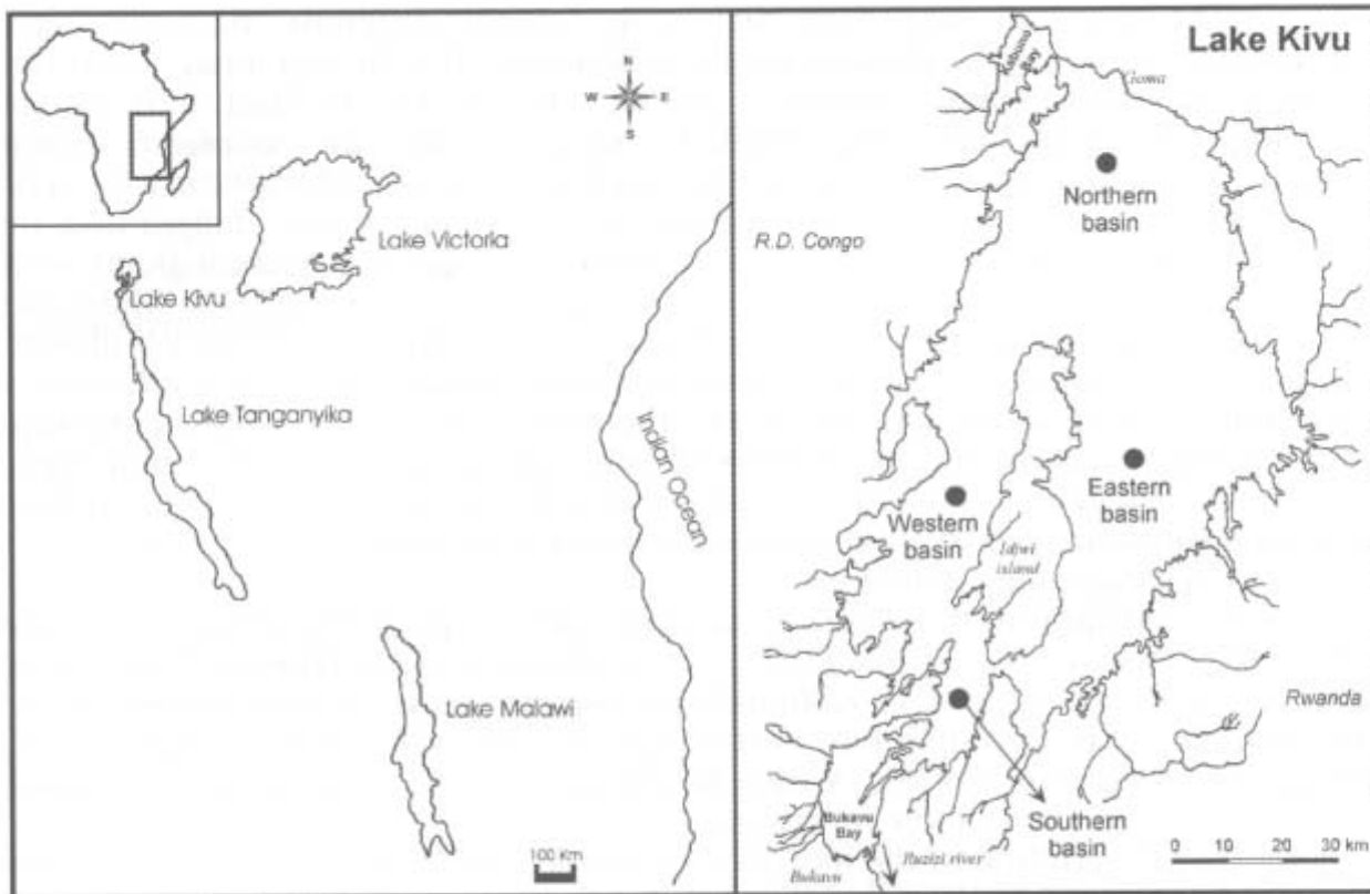
Fig. 1. Geographic situation of Lake Kivu. Black dots are the sampling sites (see text for GPS coordinates and depths).
